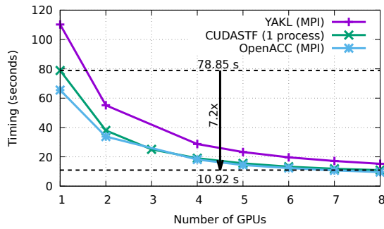
Fig. 9: Strong Scalability of miniWeather (simulation of 10000 \times 5000 elements over 10 seconds). A 7.2x speedup is measured on 8 A100s.
