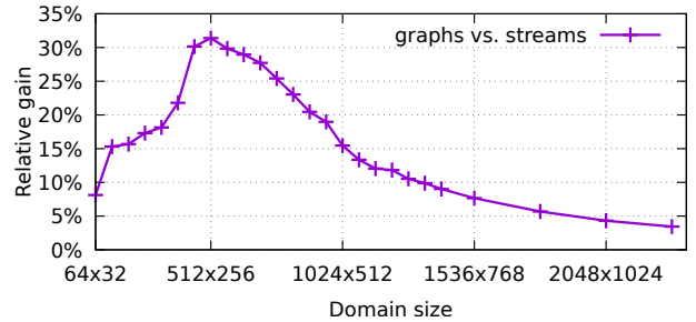
Fig. 10: Performance gains resulting from the use of CUDA graphs on small miniWeather problem sizes on one A100
