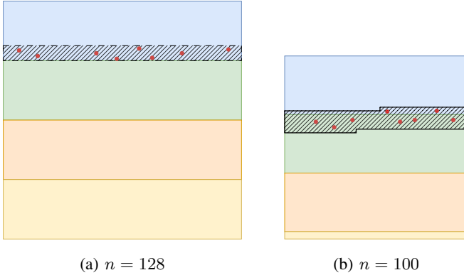
Fig. 7: Mapping of a n \times n grid with 4 KB pages and tiles of 32 lines as indicated by different colors. The fourth virtual page is hatched. With n = 128 , all 8 samples are mapped on the first device, and we observe a perfect match of the partitioner and the virtual memory mapping. With n = 100 , 2 samples are owned by the first device and the other 6 samples are owned by the second device.
