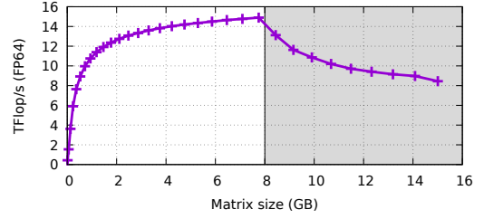
Fig. 3: Capping Cholesky decomposition at 8 GB (one A100)
