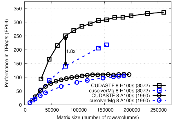
Fig. 8: Cholesky decomposition over 8 GPUs
