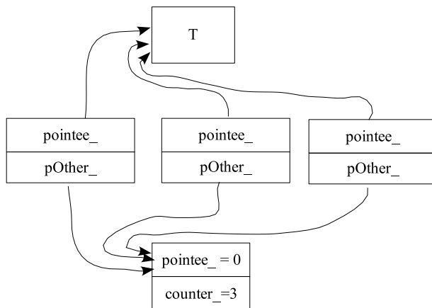
Figure 3: Third scenario. Three (or more) smart pointers are pointing to the same resource, case in which a helper smart_ptr object is conjured off the heap and used as a counter.
