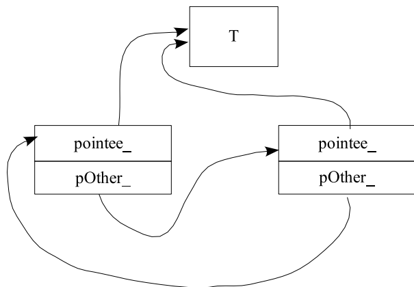
Figure 2: Second scenario. Two smart pointers pointing to the same resource
